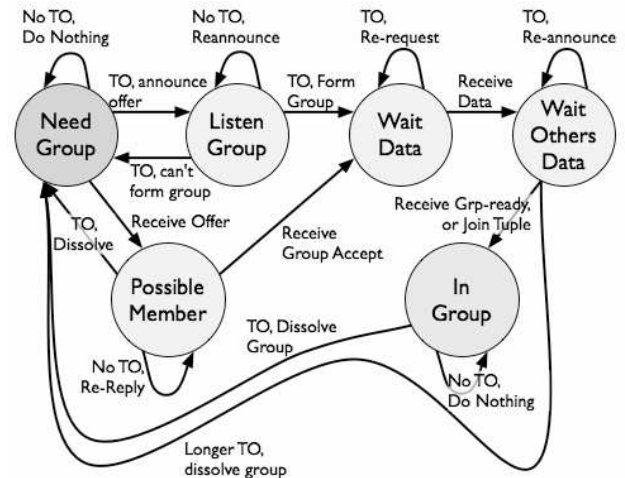
Figure 2: Join Algorithm Finite State Machine. The “TO” transitions represent timeouts, which are used to prevent deadlocks in the event of lost data or failed nodes.
